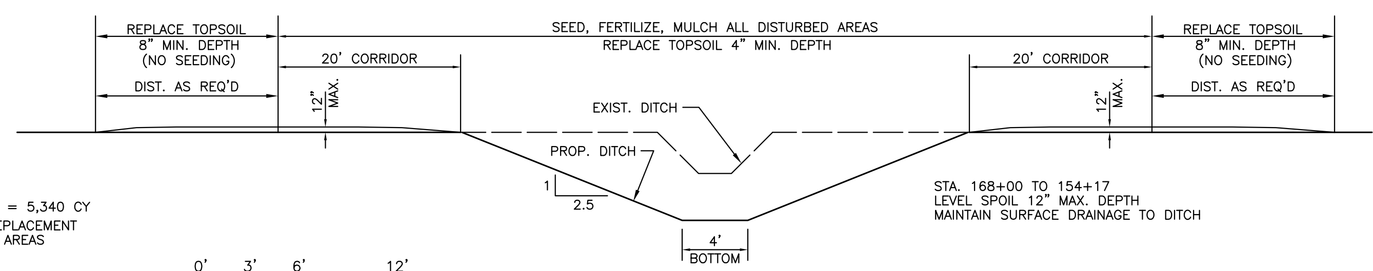
DITCH DETAIL
